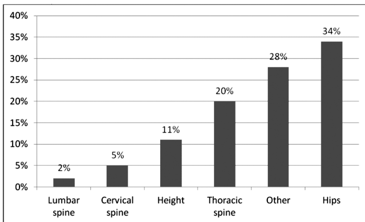
Figure 1. The values of the coefficient of determination ( R^2 ) for the tested joints in reference to the result of the EUROFIT suppleness test for the students of the Ballet School
