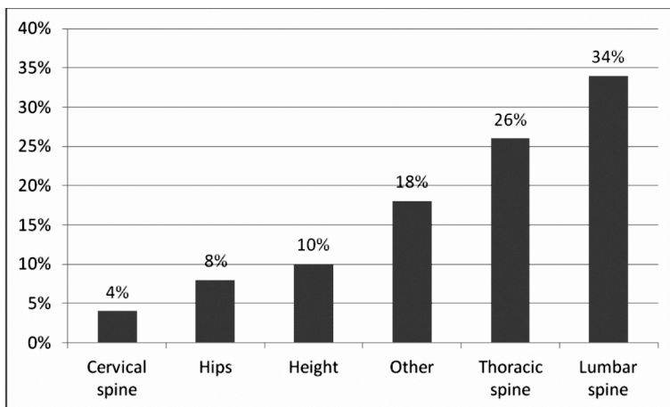
Figure 2. The values of the determination coefficient ( R^2 ) for the tested joint in reference to the result of the EUROFIT agility test for the students of the 1 st Secondary School
